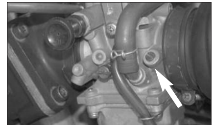
12. Locate the air mixture screw and turn clockwise until lightly seated. Now turn the screw counter clockwise 2 full turns. Note: This step will need to be repeated on both carburetors.
